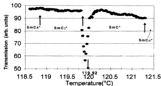
FIG. 14. Transmission of ( R )-MHPOBC (homeotropic alignment); thickness: (100 \pm 5) \mu\text{m} ; \lambda = 632.8 \text{ nm} ; wave vector of the light parallel to the layer normal.
