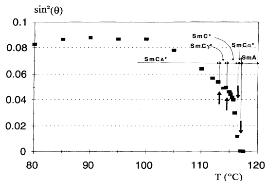
FIG. 12. Variation of \sin^2\theta ( \theta : tilt angle) vs temperature from RIA results; sample: ( R )-MHPOBC; planar geometry; thickness: (6.28 \pm 0.02) \mu\text{m} ; electric-field-induced alignment.
