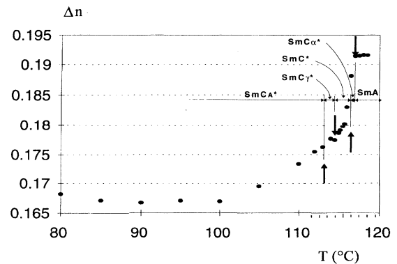
FIG. 11. RIA results; sample: ( R )-MHPOBC; planar geometry; thickness: (6.28 \pm 0.02)\text{ }\mu\text{m} ; electric-field-induced alignment.
